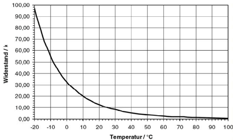
Abb.30 Diagramm (Widerstand in kΩ)
